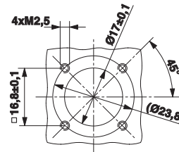
Dimensional drawing
